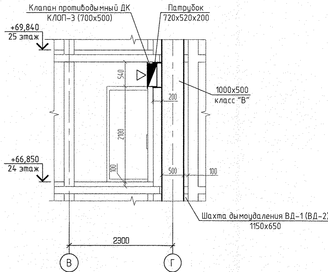
7 - 7 (1:50)
