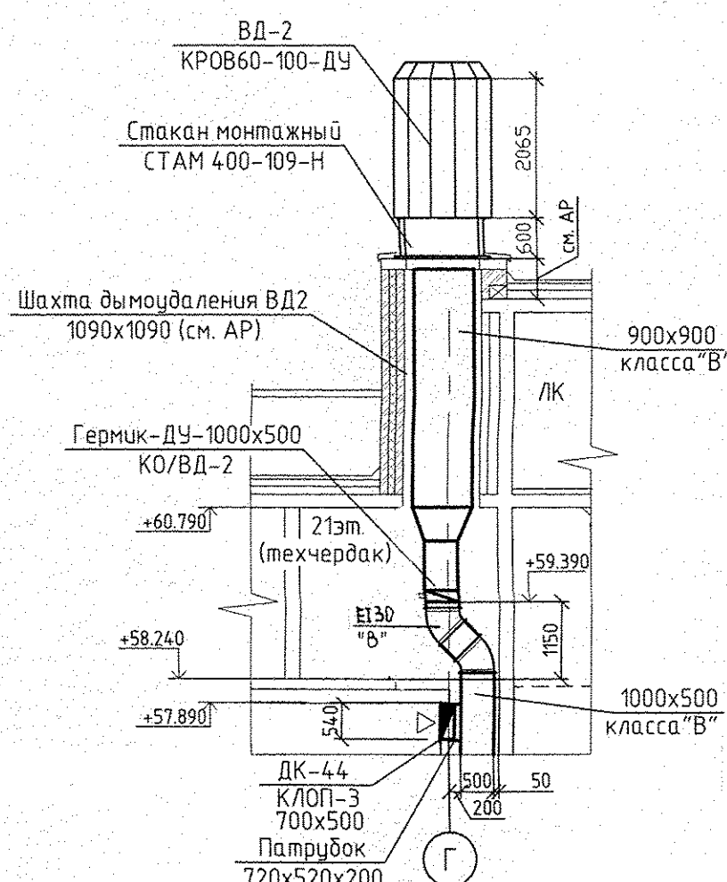
5 - 5 (1:100)
