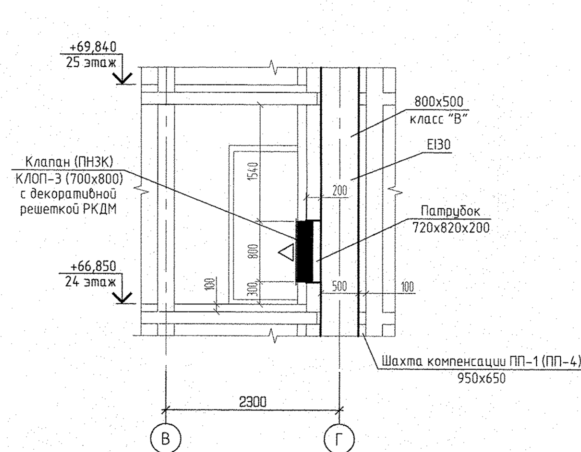
8 - 8 (1:50)
