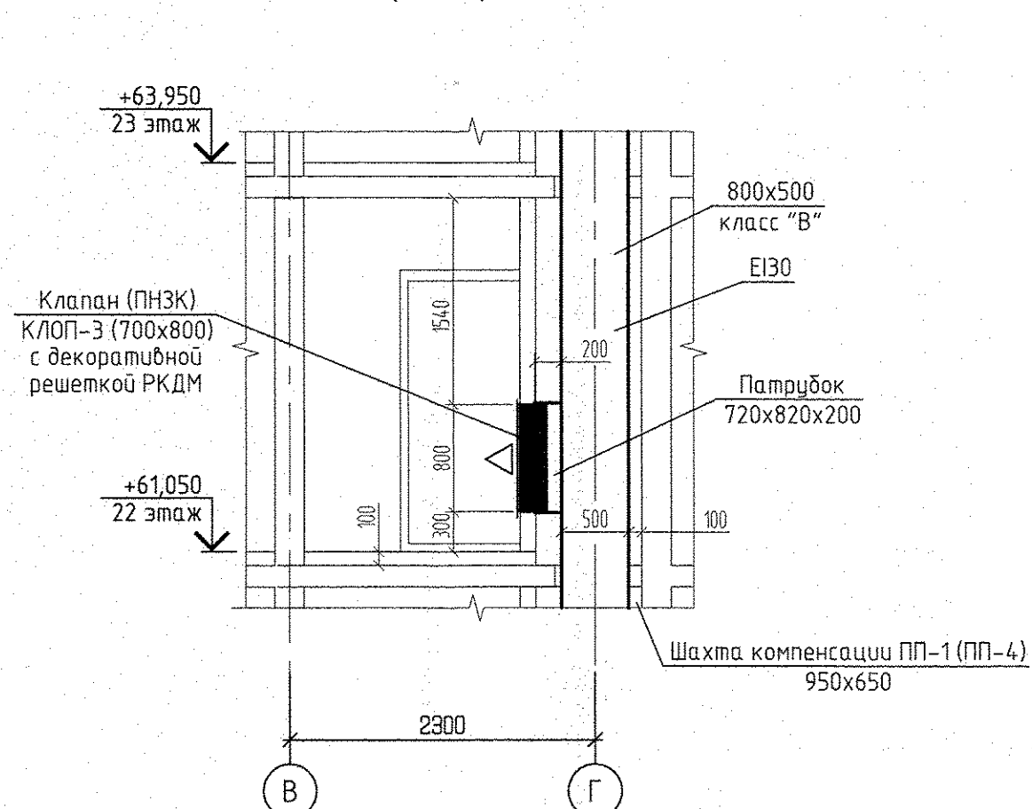
8 - 8 (1:50)
