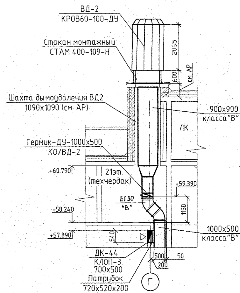
5 - 5 (1:100)
