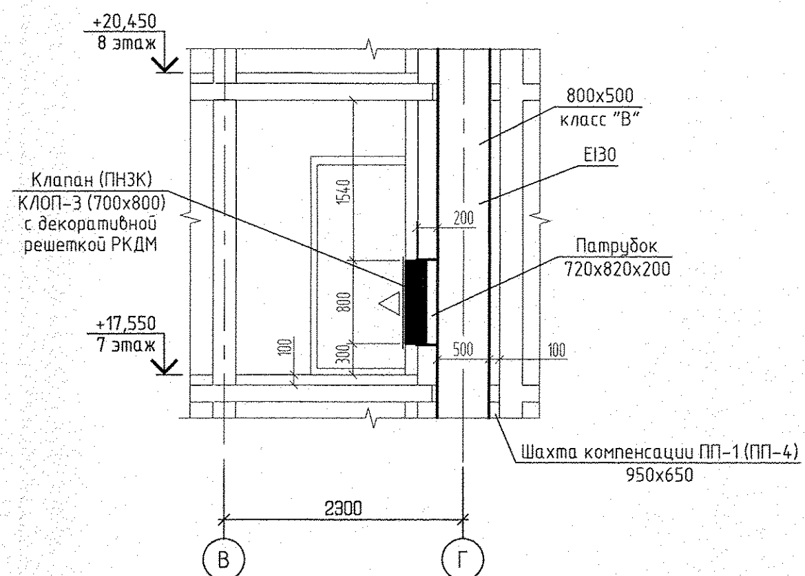
2 - 2 (1:50)
