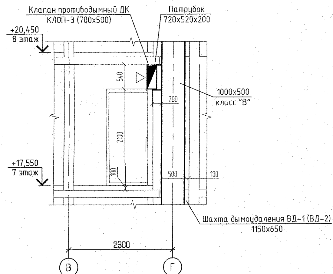
1 - 1 (1:50)
