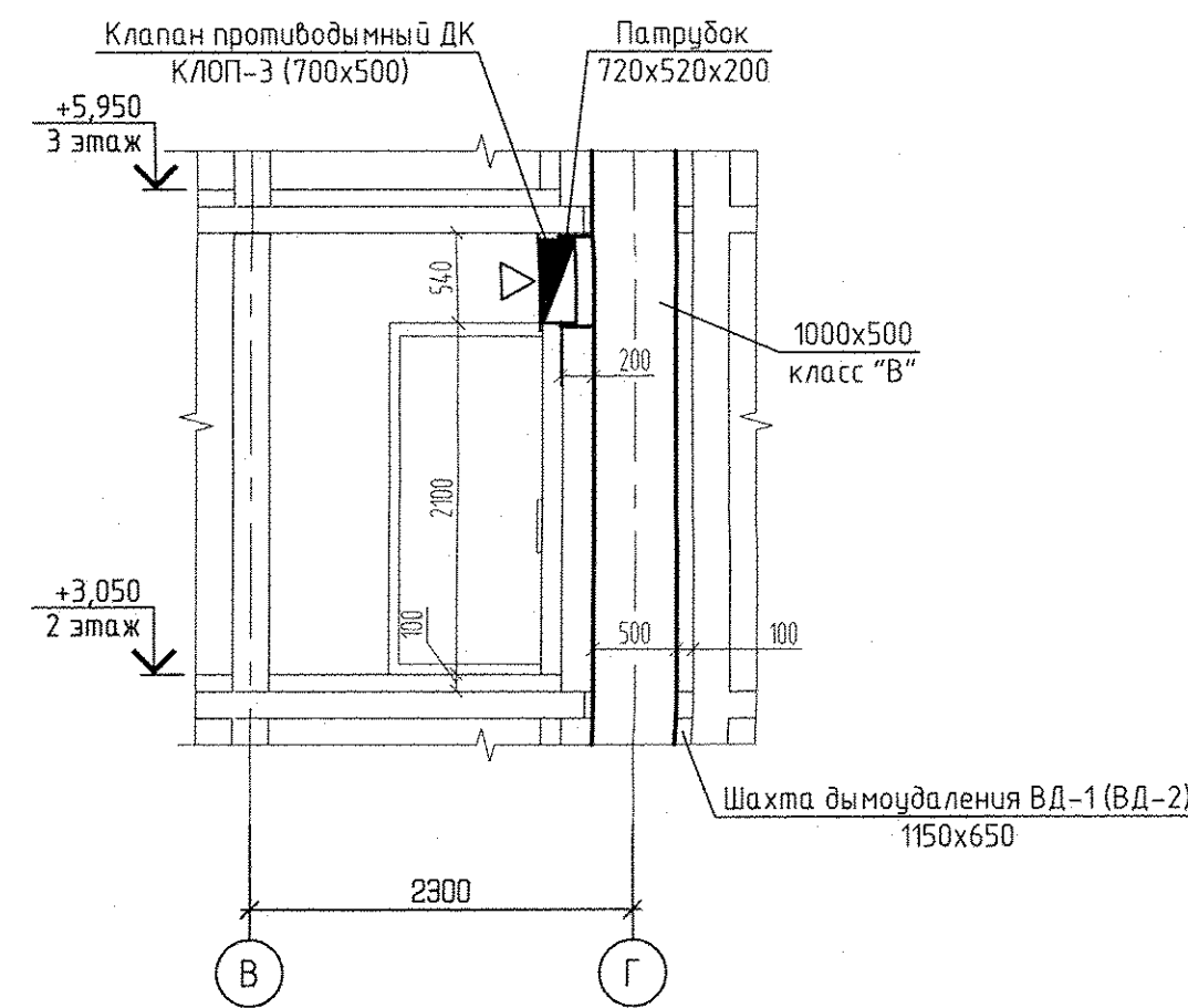
1-1 (1:50)
