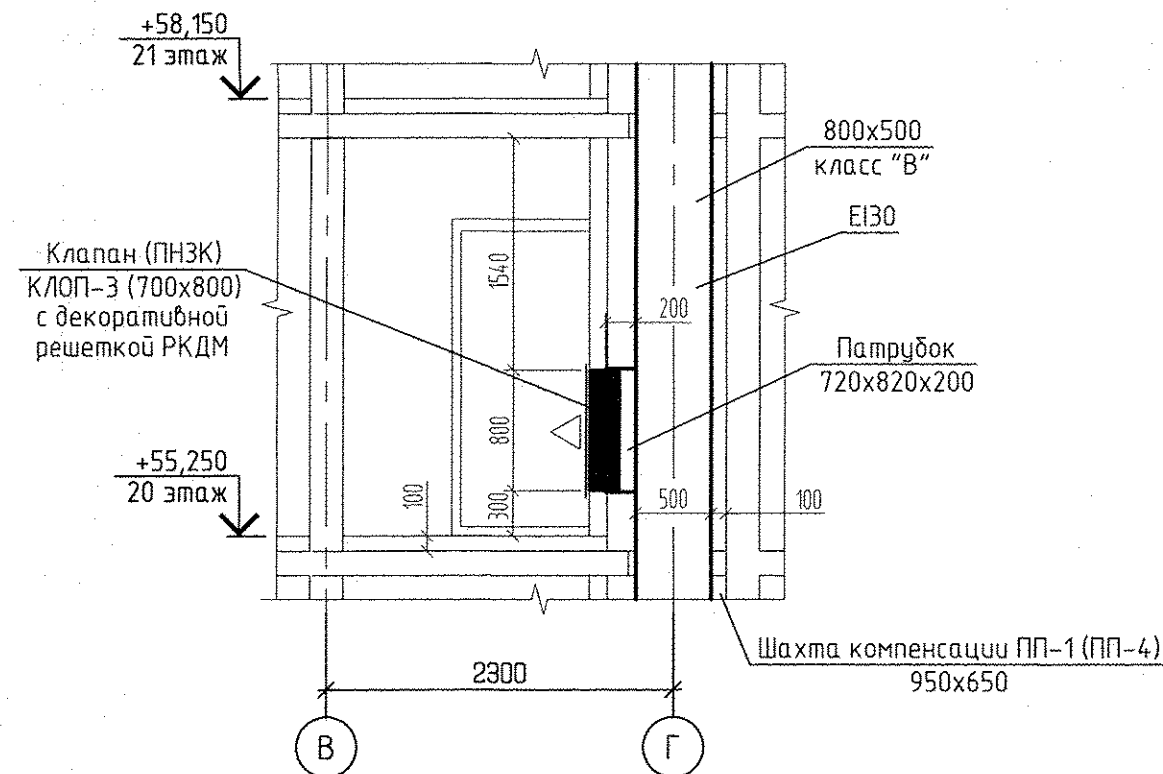
2-2 (1:50)
