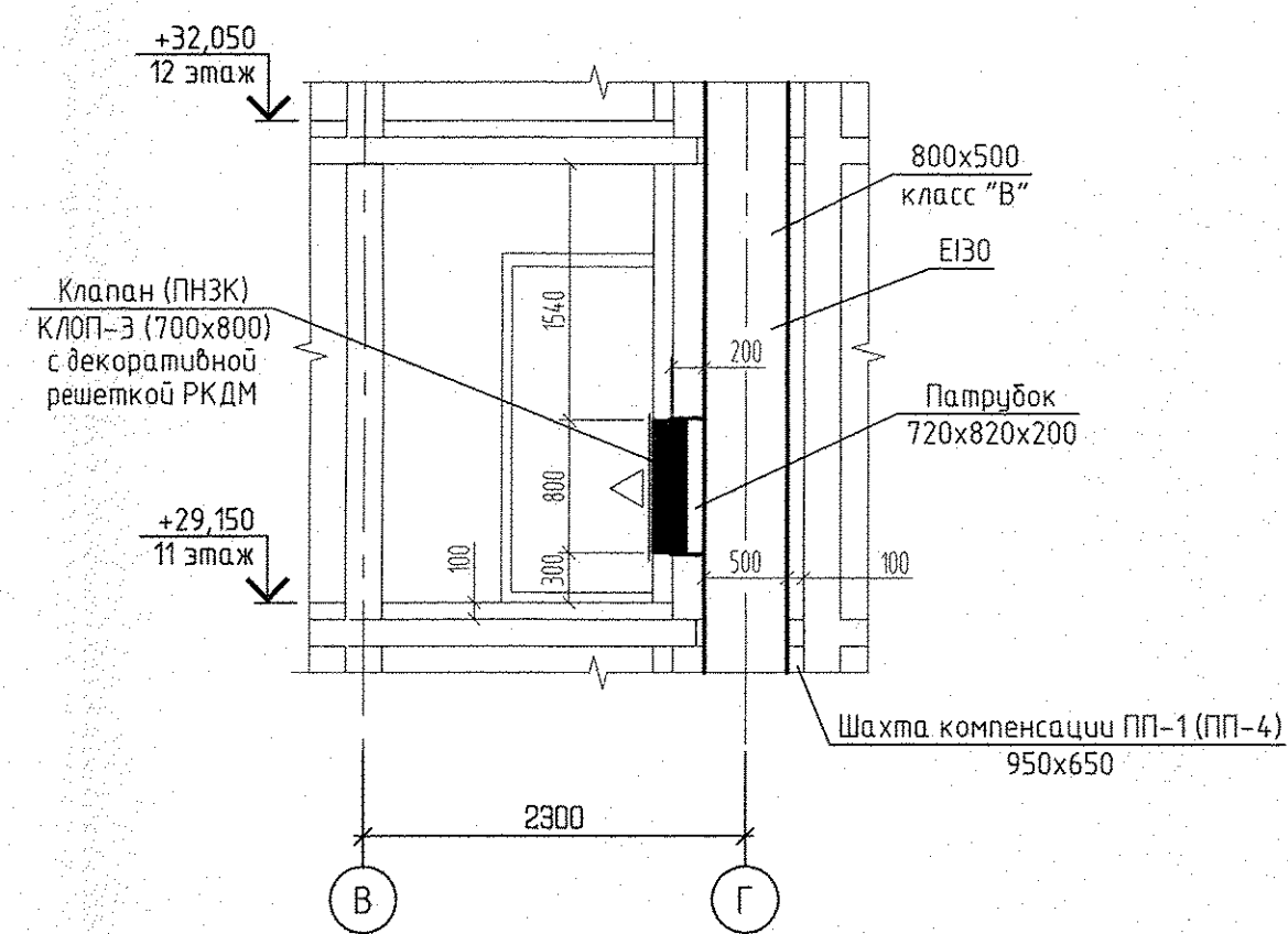
2 - 2 (1:50)
